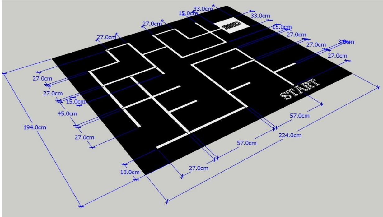
FIG 1 : Isometric View
